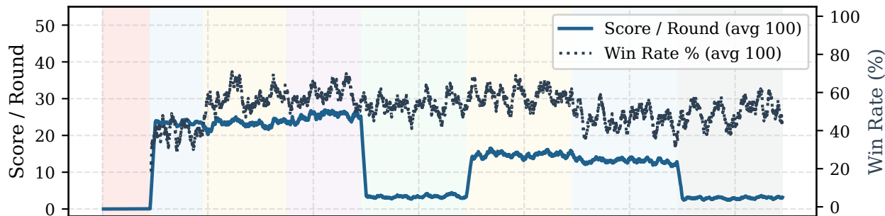
(c) Survival & Suicide Suppression under World Model Grounding
