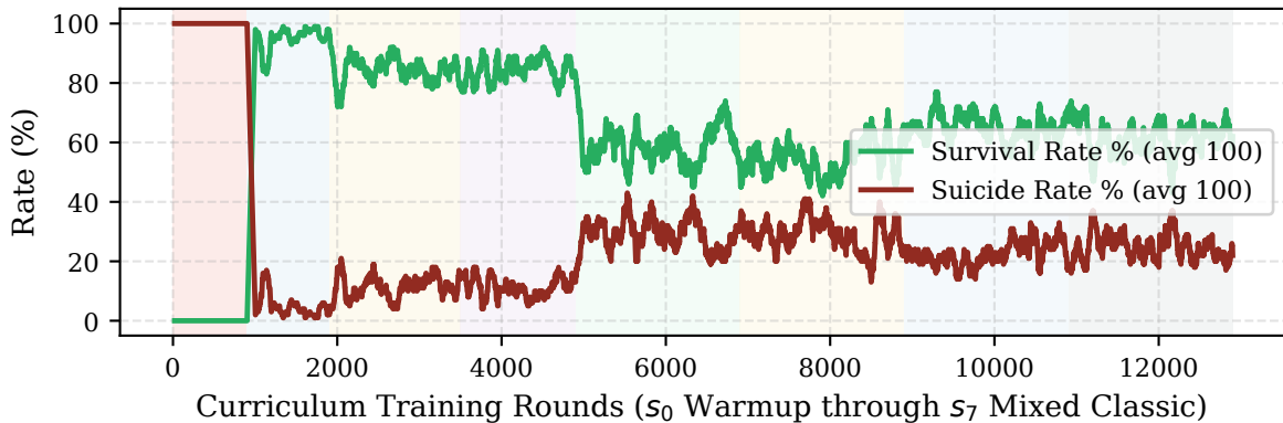
(c) Survival & Suicide Suppression under World Model Grounding
